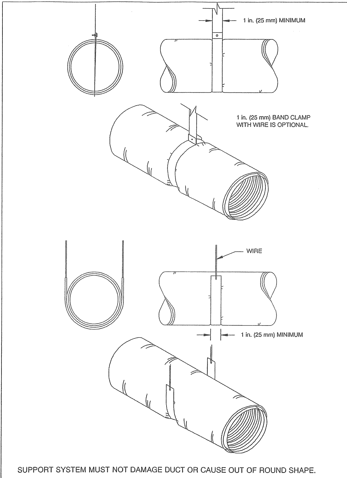
FIGURE 3-11 FLEXIBLE DUCT SUPPORTS
