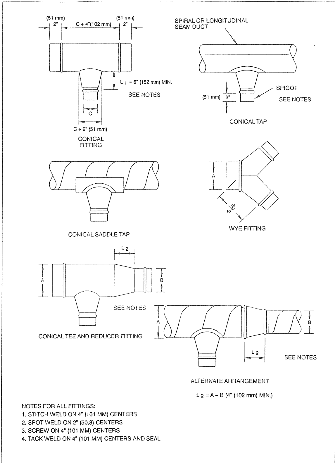
FIGURE 3-6 CONICAL TEES
