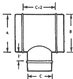
STRAIGHT TEE
