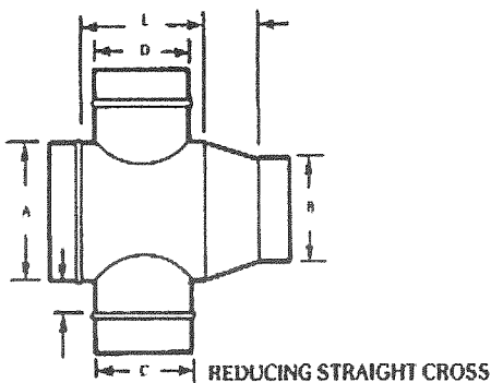
REDUCING STRAIGHT CROSS
