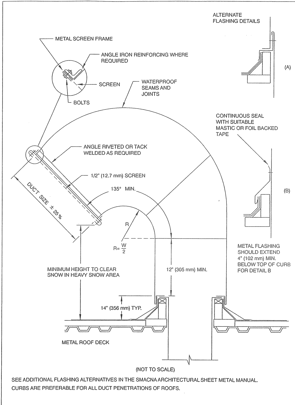
FIGURE 6-5 RECTANGULAR GOOSENECK
